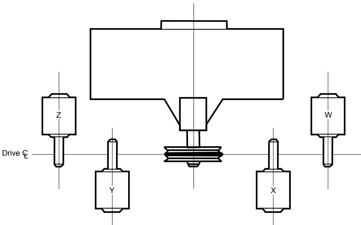
Figure 1: Plan View Of A Centrifugal Fan
