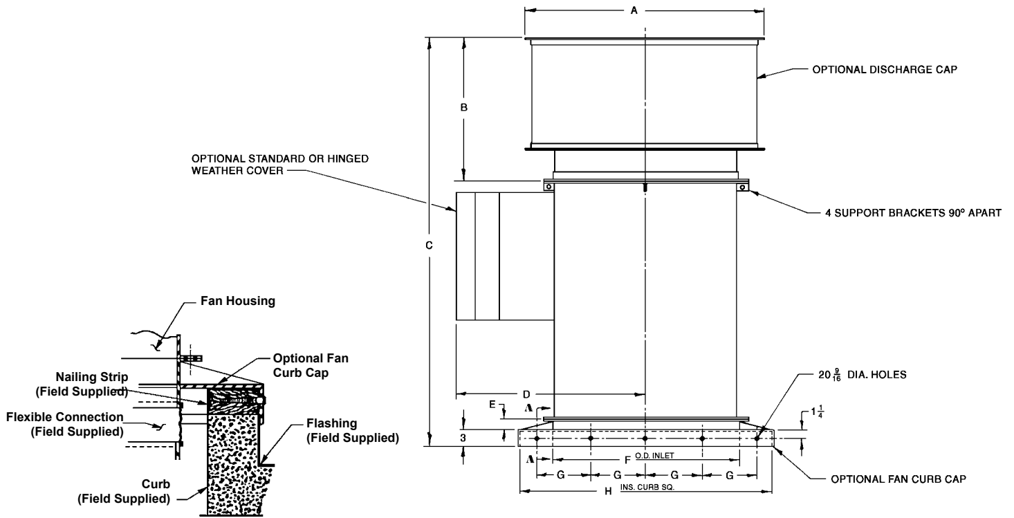
SECTION A-A Recommended Curb Construction
