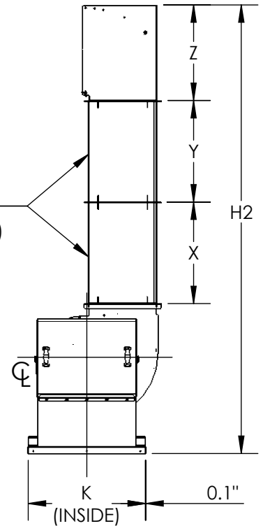
FAN WITH OPTIONAL STACK EXTENSION
