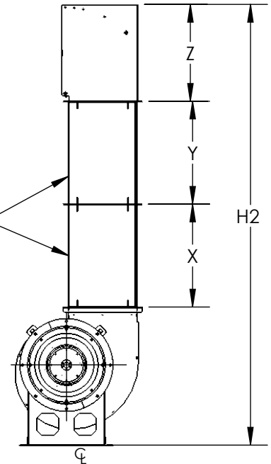
FAN WITH OPTIONAL STACK EXTENSION
