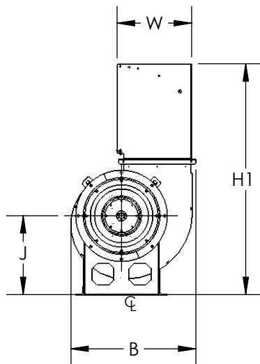
INLET SIDE VIEW
