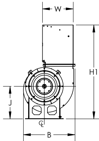
INLET SIDE VIEW
