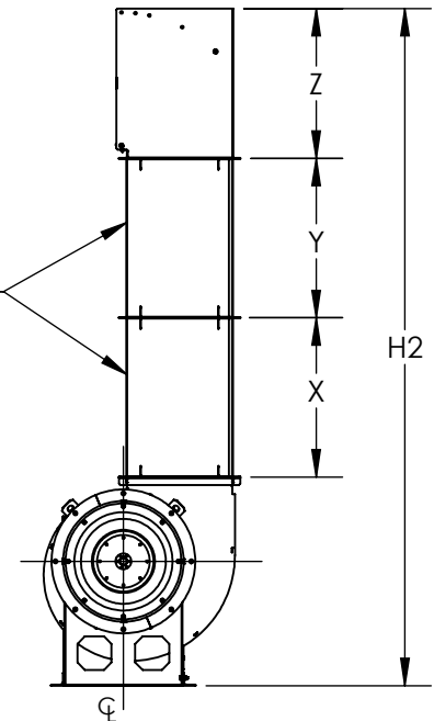
FAN WITH OPTIONAL STACK EXTENSION
