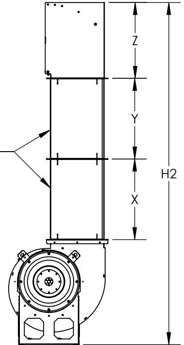
FAN WITH OPTIONAL STACK EXTENSION
