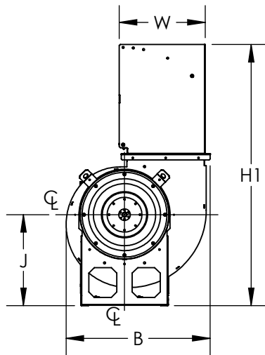
INLET SIDE VIEW
