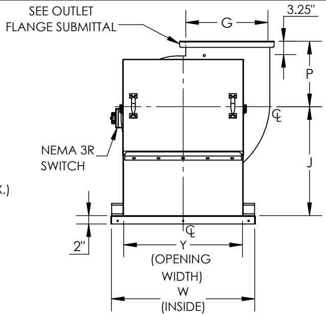
INLET VIEW
