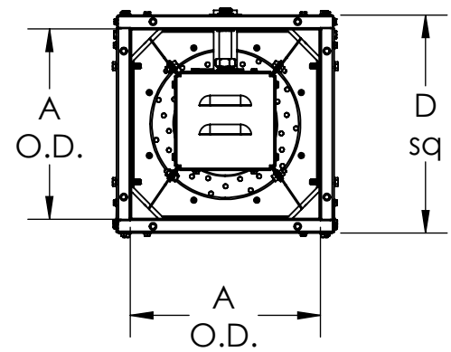
DISCHARGE VIEW
