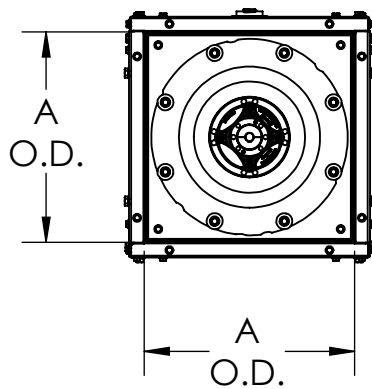
INLET VIEW
