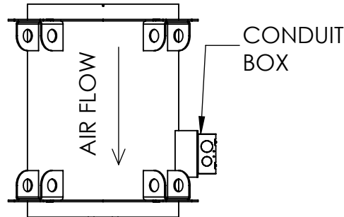
VERTICAL DOWNBLAST
