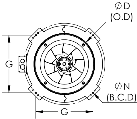
INLET VIEW
