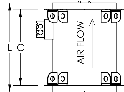
VERTICAL UPBLAST
