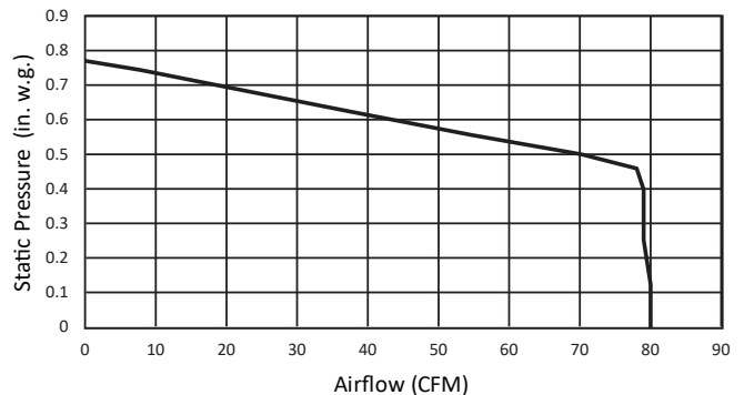
6" Duct
