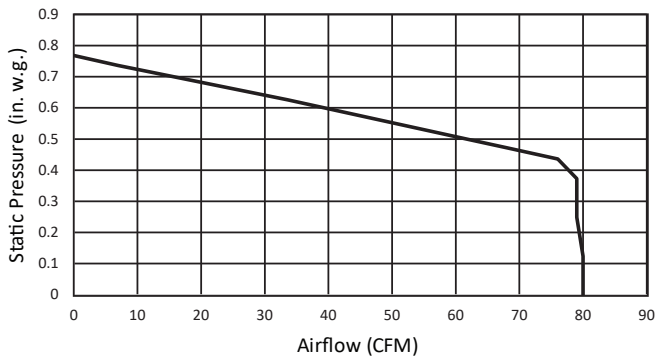
4" Duct
