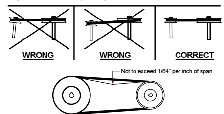
Figure 2: Pulley Alignment
